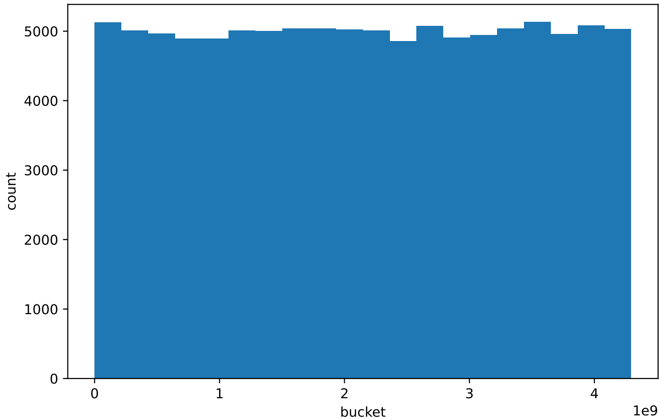
Xorshift32 good histogram
