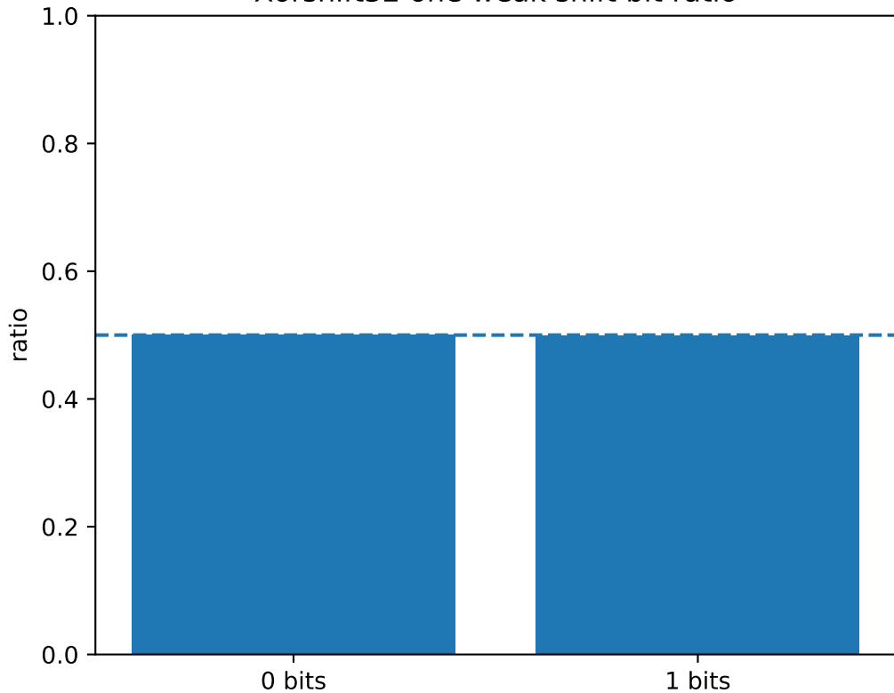
Xorshift32 one weak shift bit ratio
