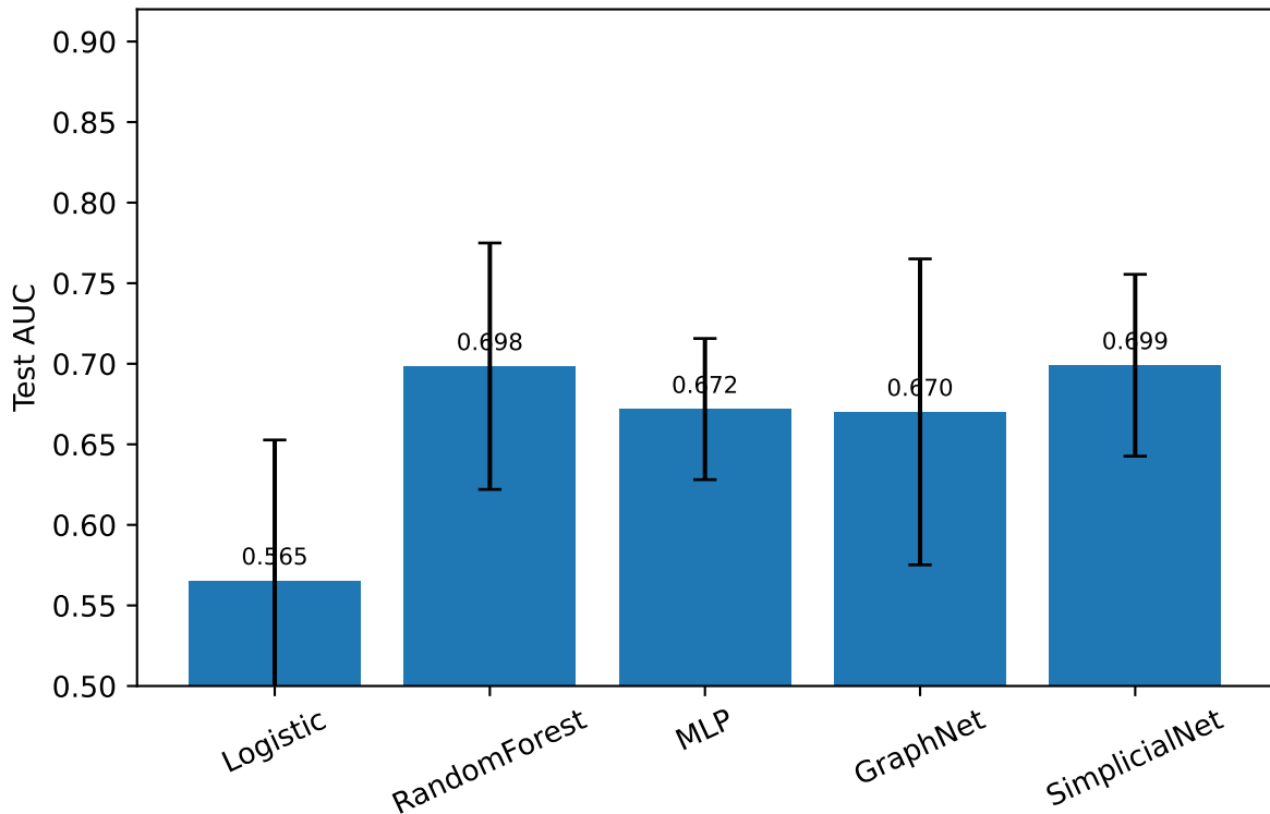
Demonstration output: topology-aware models improve ranking performance
