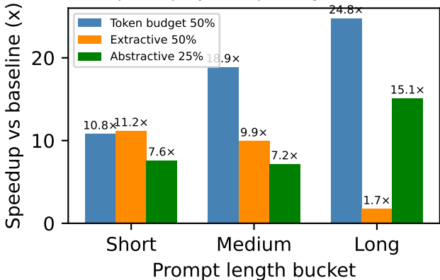
Speedup by Prompt Length Bucket
