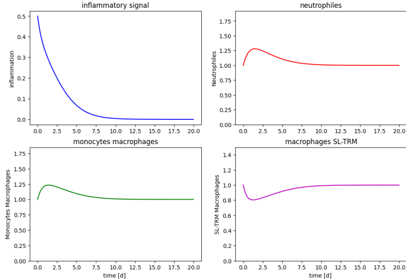
Figure 10: A=0.38, S(0)=0.5
