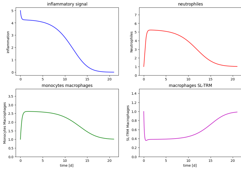
Figure 12: A=0.072 , S(0)=5
