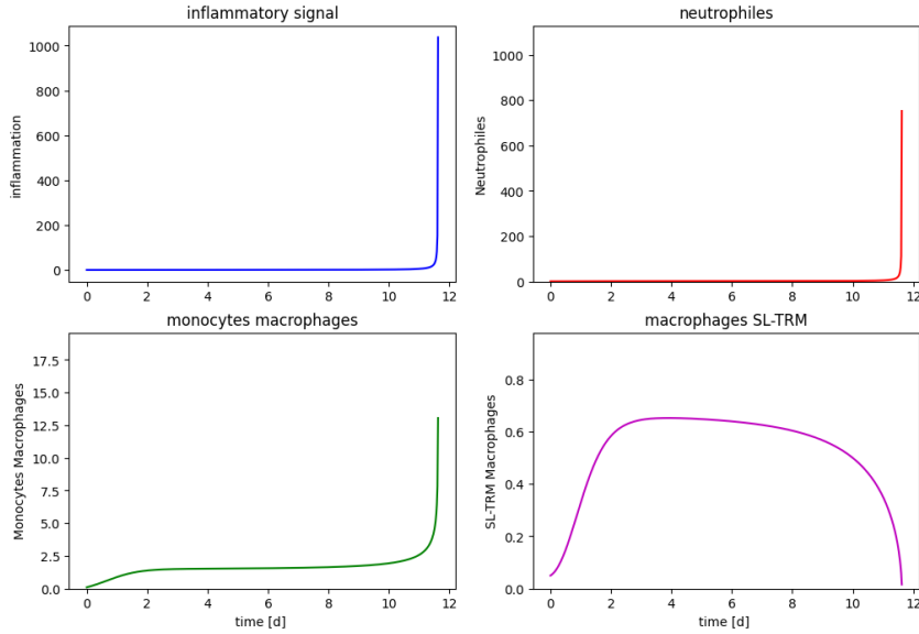
Figure 7: A = 0.38, S(0) = 0.5 , immunocompromised initial conditions, crisis escalation.
