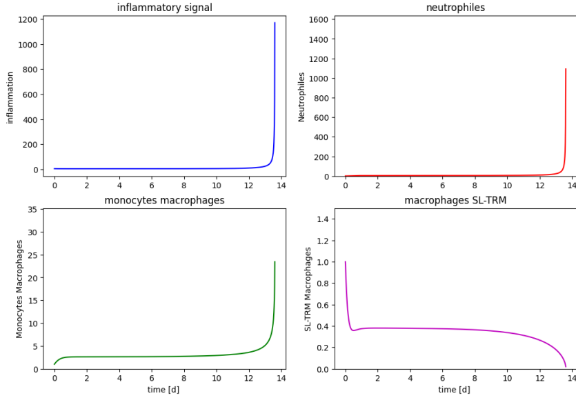
Figure 9: A = 0.073 , S(0) = 5 (high dose of immune signal), crisis escalation.
