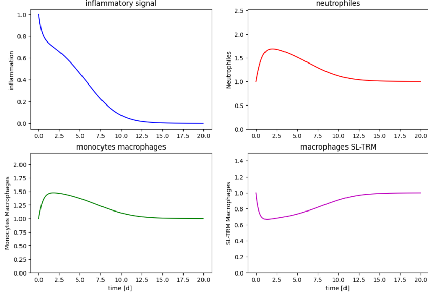
Figure 4: A = 0.35 , crisis resolution.
