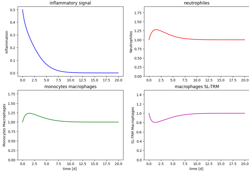
Figure 6: A = 0.38, S(0) = 0.5 (half dose of immune signal), crisis resolution.
