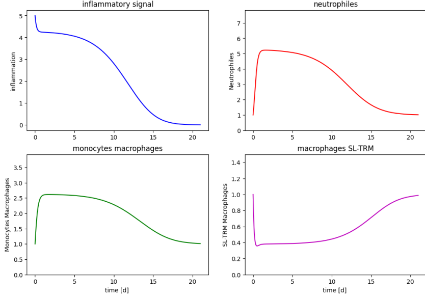
Figure 8: A = 0.072 , S(0) = 5 (high dose of immune signal), crisis resolution.
