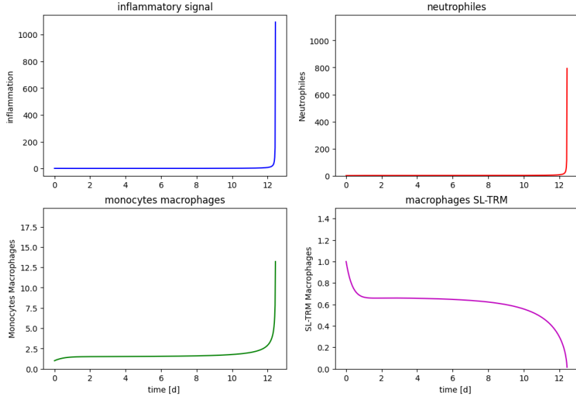
Figure 5: A = 0.38 , crisis escalation.
