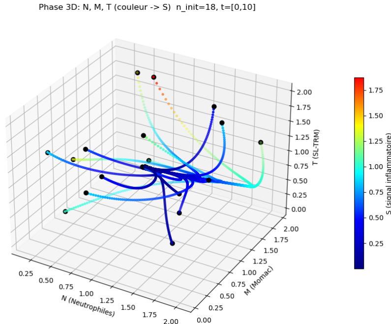
Figure 13: Phase space trajectory in the (S, N, M, T) space, S intensity corresponds to the color scale.
