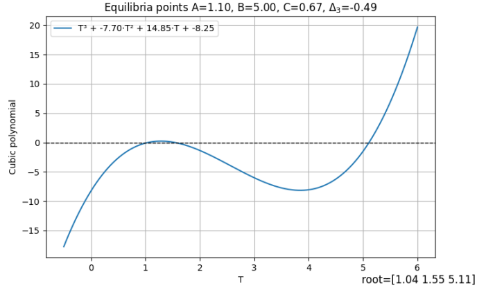
Figure 5: Cubic equation with three distinct real roots.
