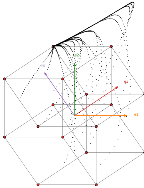
Figure 14: 2D projections of the 4D phase space trajectory using the tesseract representation.
