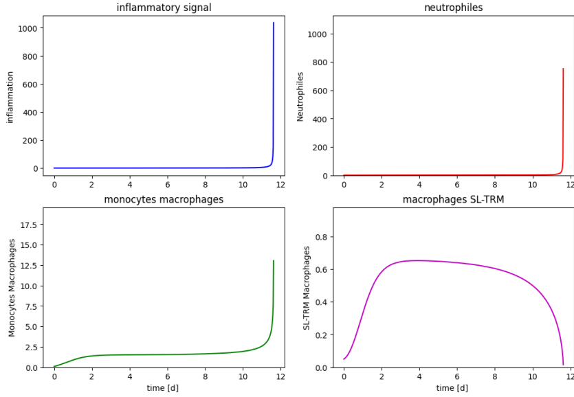
Figure 8: A=0.38 , immunocompromised initial conditions
