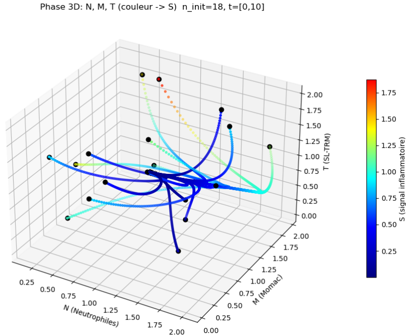
Figure 12: Phase space trajectory in the (S, N, M, T) space, S intensity corresponds to the color scale.
