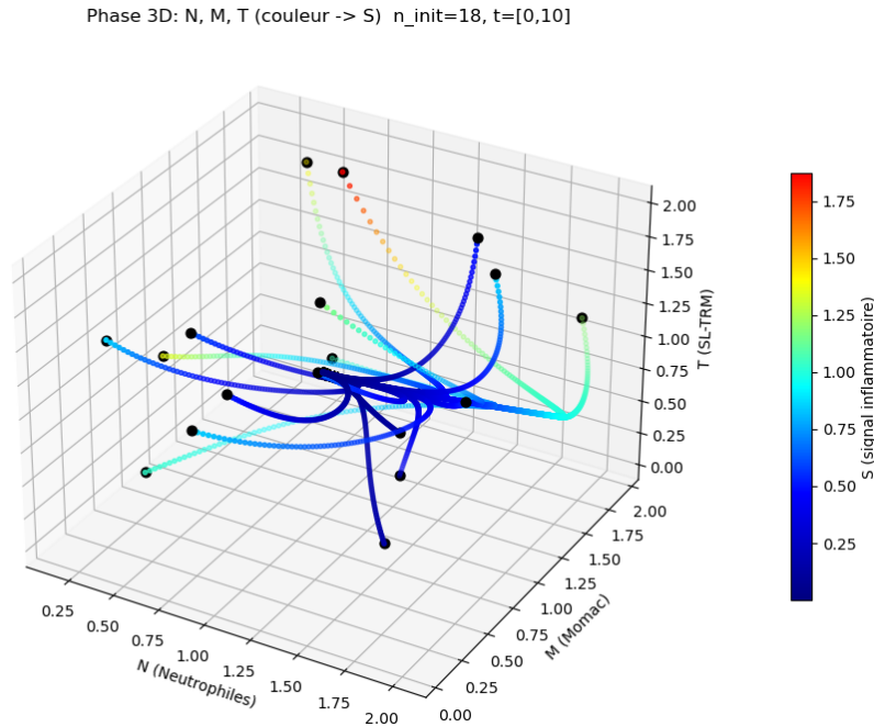
Figure 8: Phase space trajectory in the (S, N, M, T) space.
