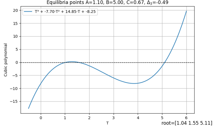
Figure 3: Cubic equation with three distinct real roots.
