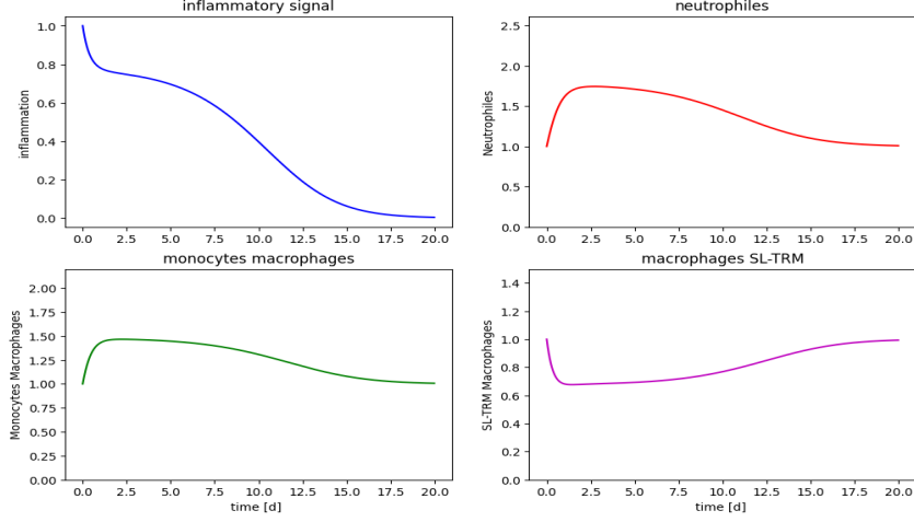
Figure 8: A = 0.072, S(0) = 5, A = 0.38, \delta_M = 1.1 (increased regulation of MoMac/SL-TRM), crisis resolution.
