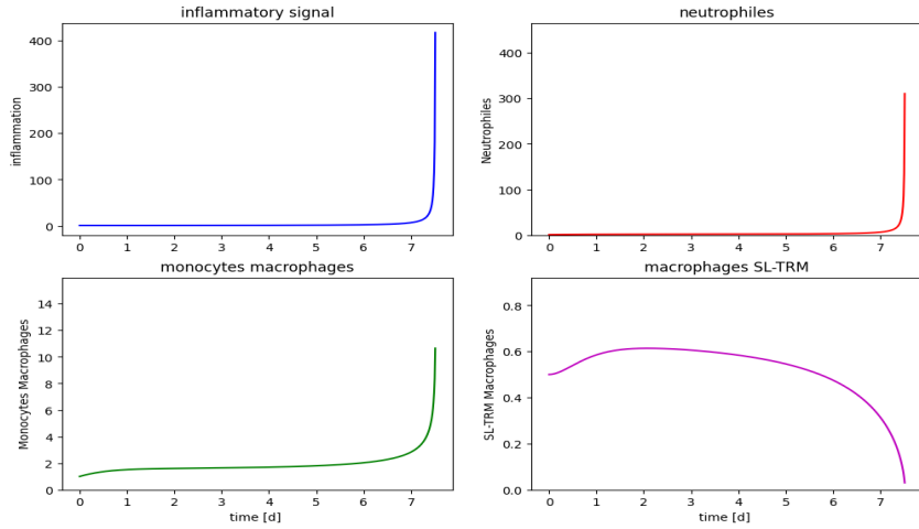
Figure 7: A = 0.38 , immunocompromised A = 0.35, T(0) = 0.5 (depleted initial conditions population of SL-TRM), crisis escalation.
