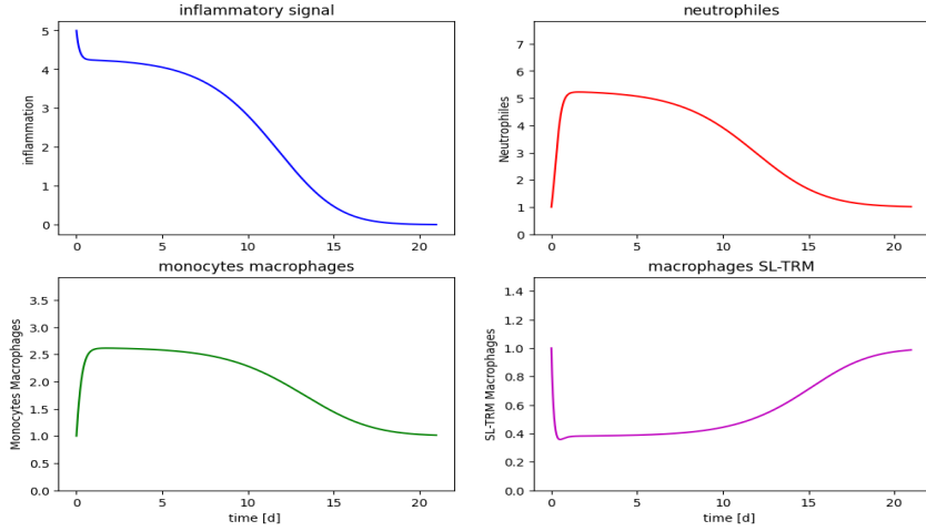
Figure 9: A = 0.073, S(0) = 5, A = 0.072, S(0) = 5 (high dose of immune signal), crisis resolution.
