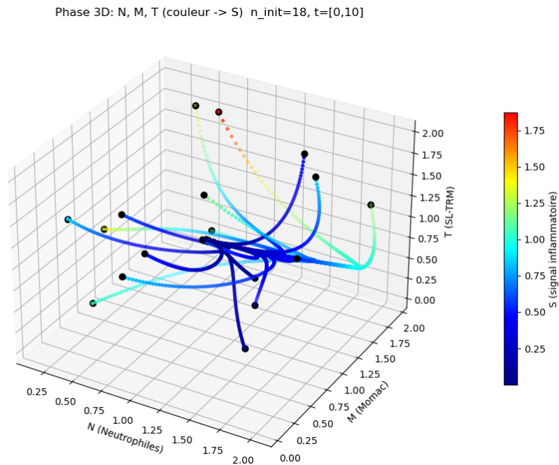
Figure 8: Phase space trajectory in the (S, N, M, T) space, S intensity corresponds to the color scale.
