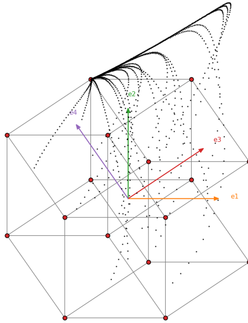
Figure 9: 2D projections of the 4D phase space trajectory using the tesseract representation.
