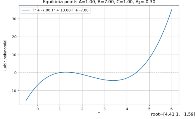
Figure 6: Cubic equation with three distinct real roots.
