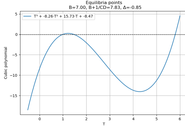
Figure 4: Cubic equation with three distinct real roots.
