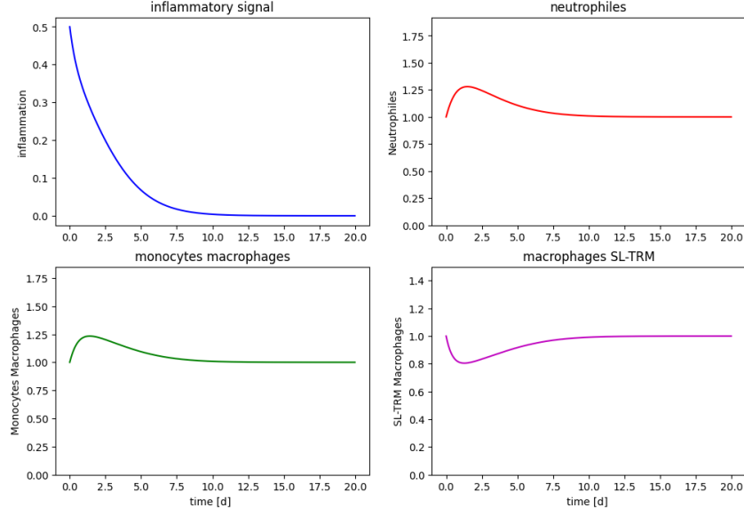
Figure 10: A=0.38 , S(0)=0.5
