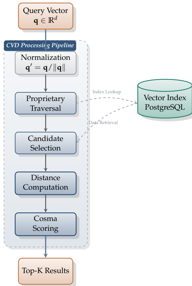
Figure 2: CVD Query Execution Pipeline - Deterministic Search Flow
