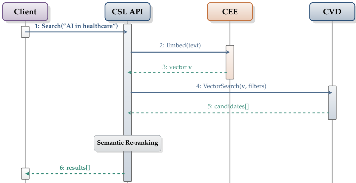
Figure 5: CSL Search Sequence - End-to-End Query Processing Flow
