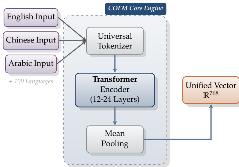
Figure 3: COEM Model Architecture - Unified Cross-Lingual Latent Space
