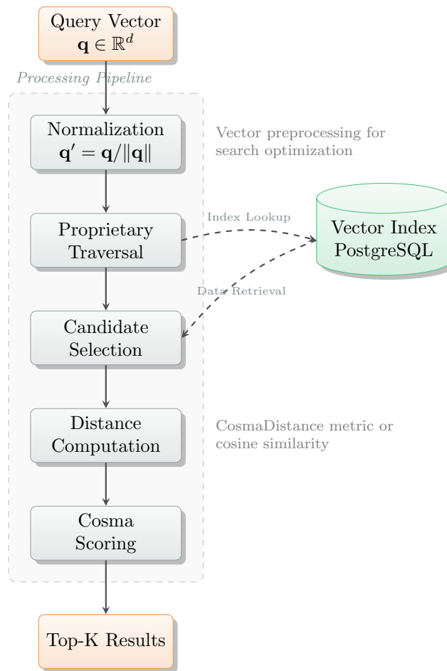
Figure 3: CVD Query Execution Pipeline
