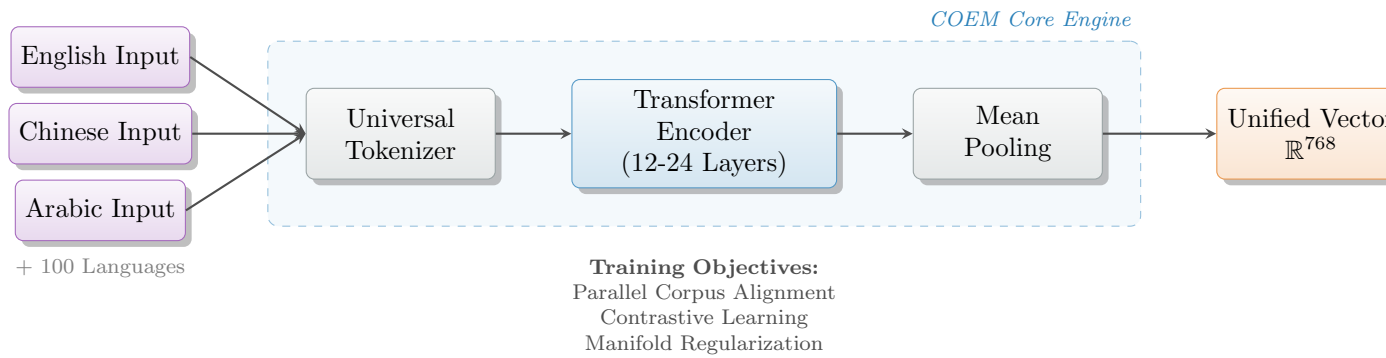
Figure 4: COEM Model Architecture - Unified Latent Space
