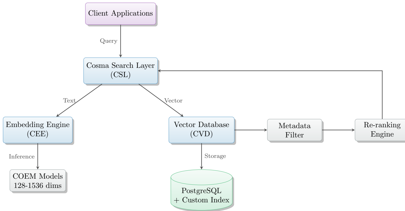
Figure 2: Component Interaction Diagram
