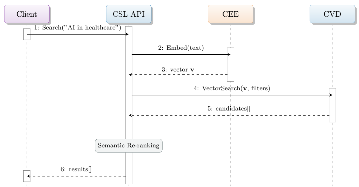
Figure 6: CSL Search Sequence Diagram
