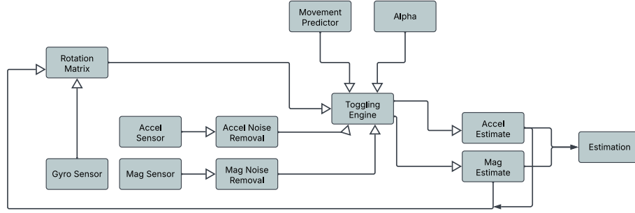
Figure 3.2: Filter Diagram
