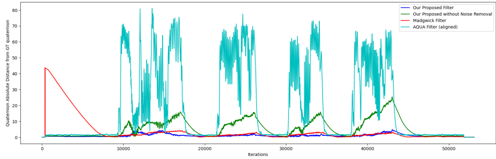
Figure 5.6: 18_undisturbed_fast_translation_with_breaks_B
