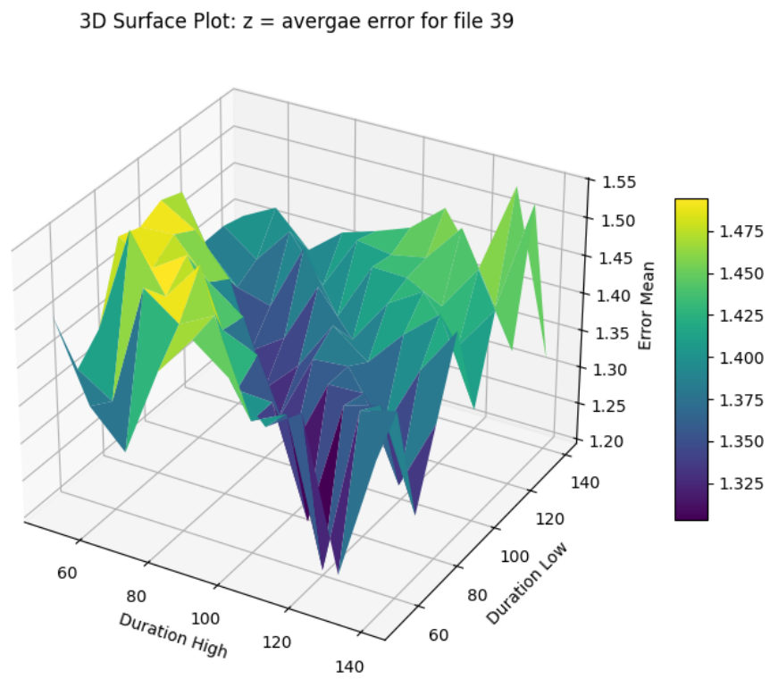
Figure 4.2: Grid search results for hyperparameter tuning of d_h and d_l . The optimal configuration corresponds to d_h = 120 and d_l = 60 .
