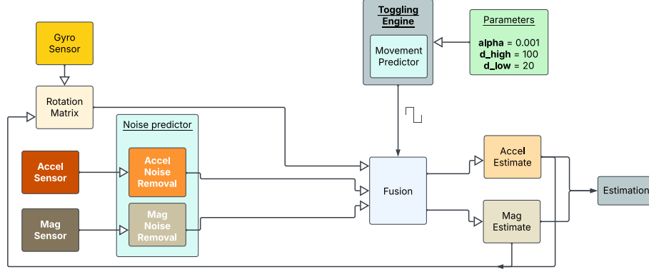
Figure 3.2: Filter Diagram 1 for our proposed Data Driven Toggling Gain CF.
