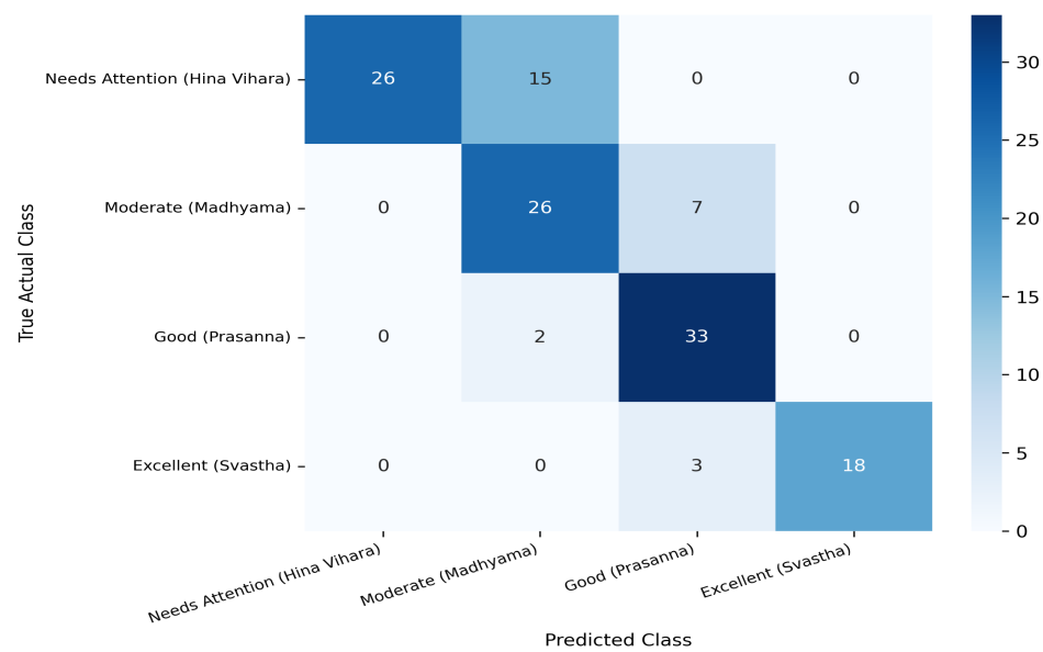
Fig. 2. Confusion Matrix: Random Forest Classifier on Holdout Test Set (N=130)
