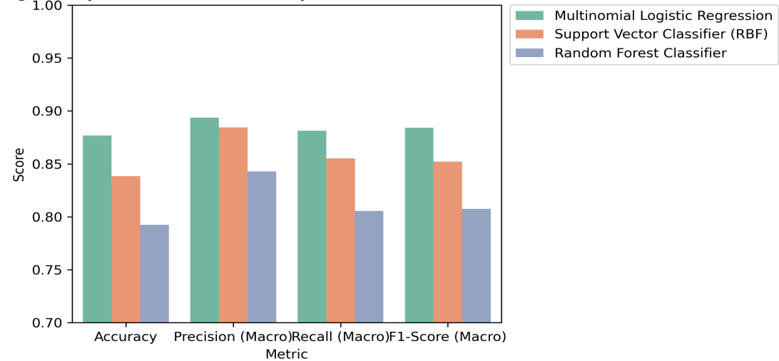
Fig. 4. Empirical Performance Comparison Across Baseline Models
