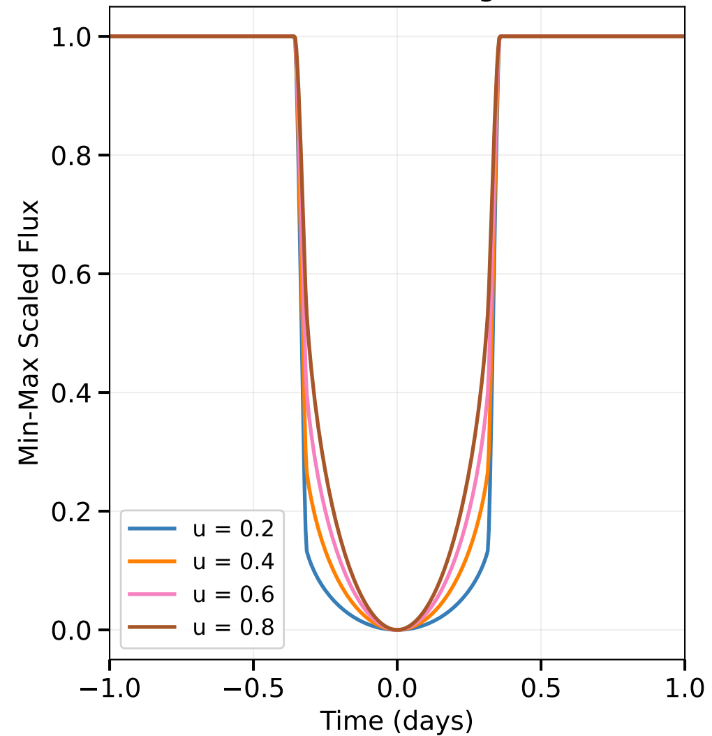
Effect of Limb Darkening ( P = 700\text{d} )
