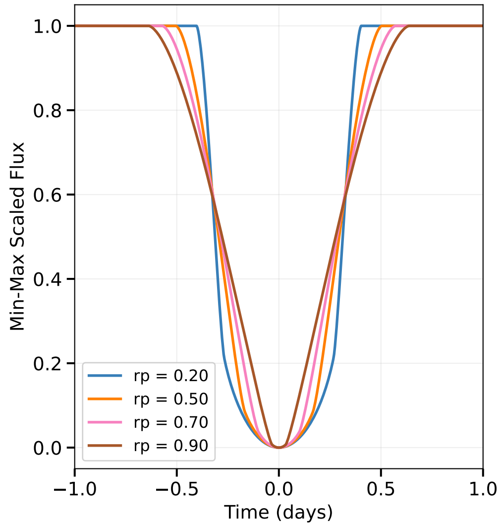
Effect of Radius ( P = 700\text{d} )
