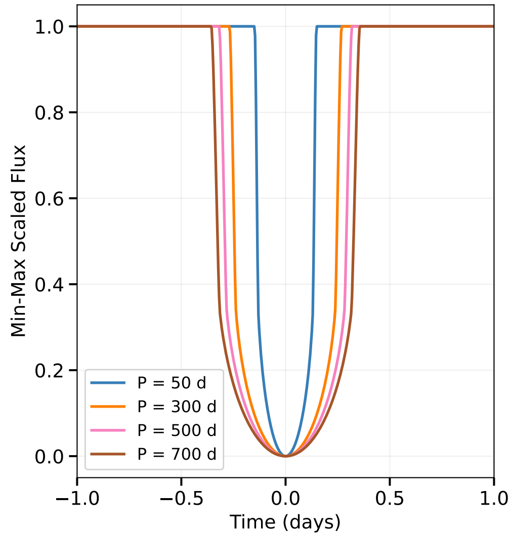
Effect of Orbital Period
