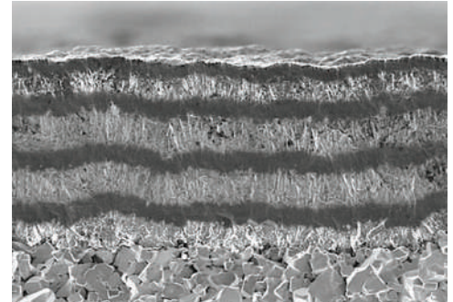
Multilayer Diamond Coating
