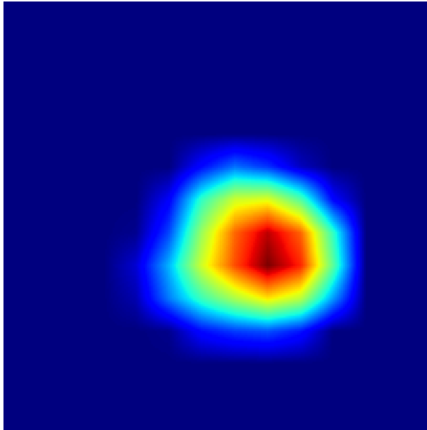
Grad-CAM Heatmap
