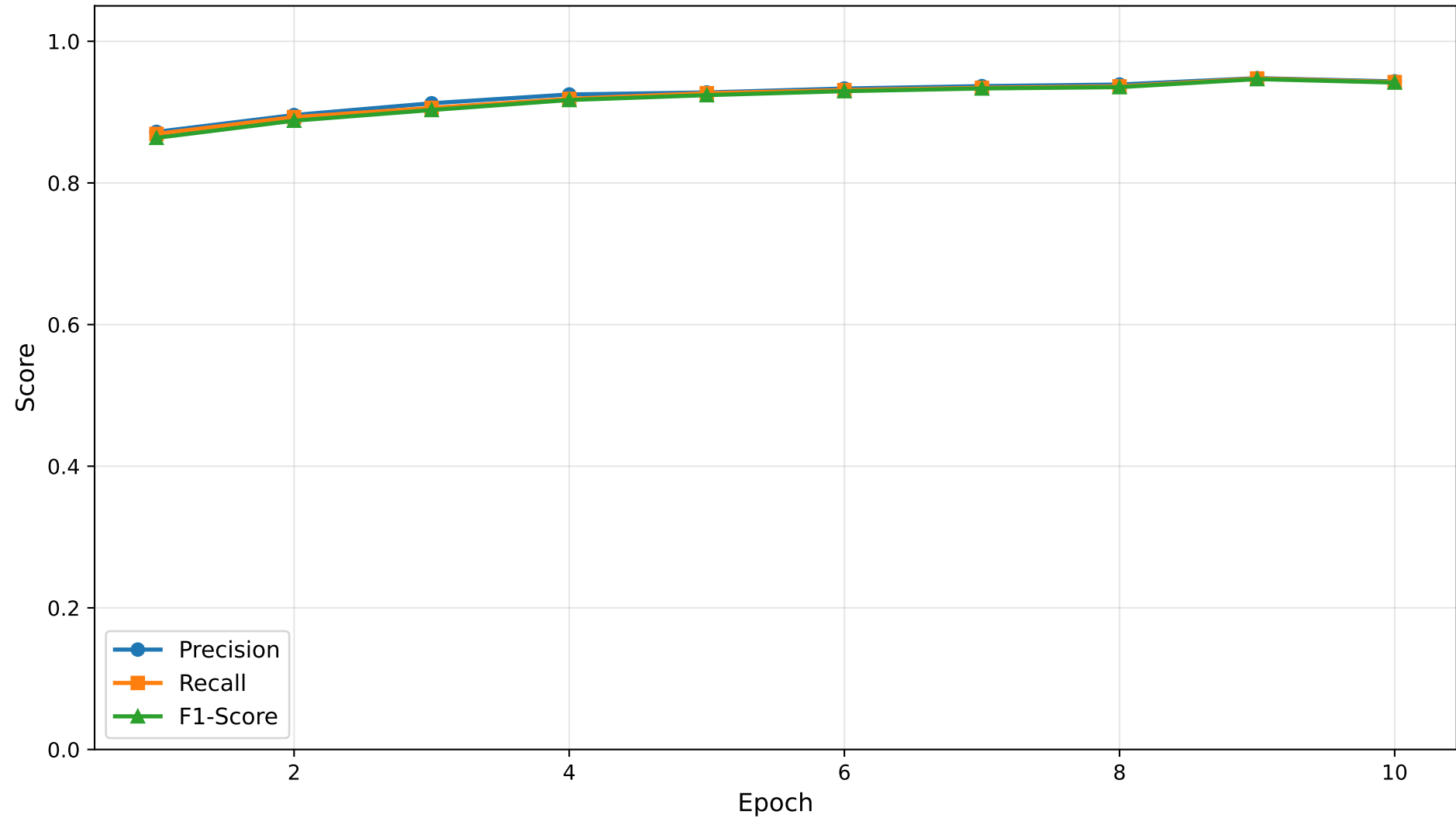
RQ2 Fig 2: Validation Metrics Evolution
