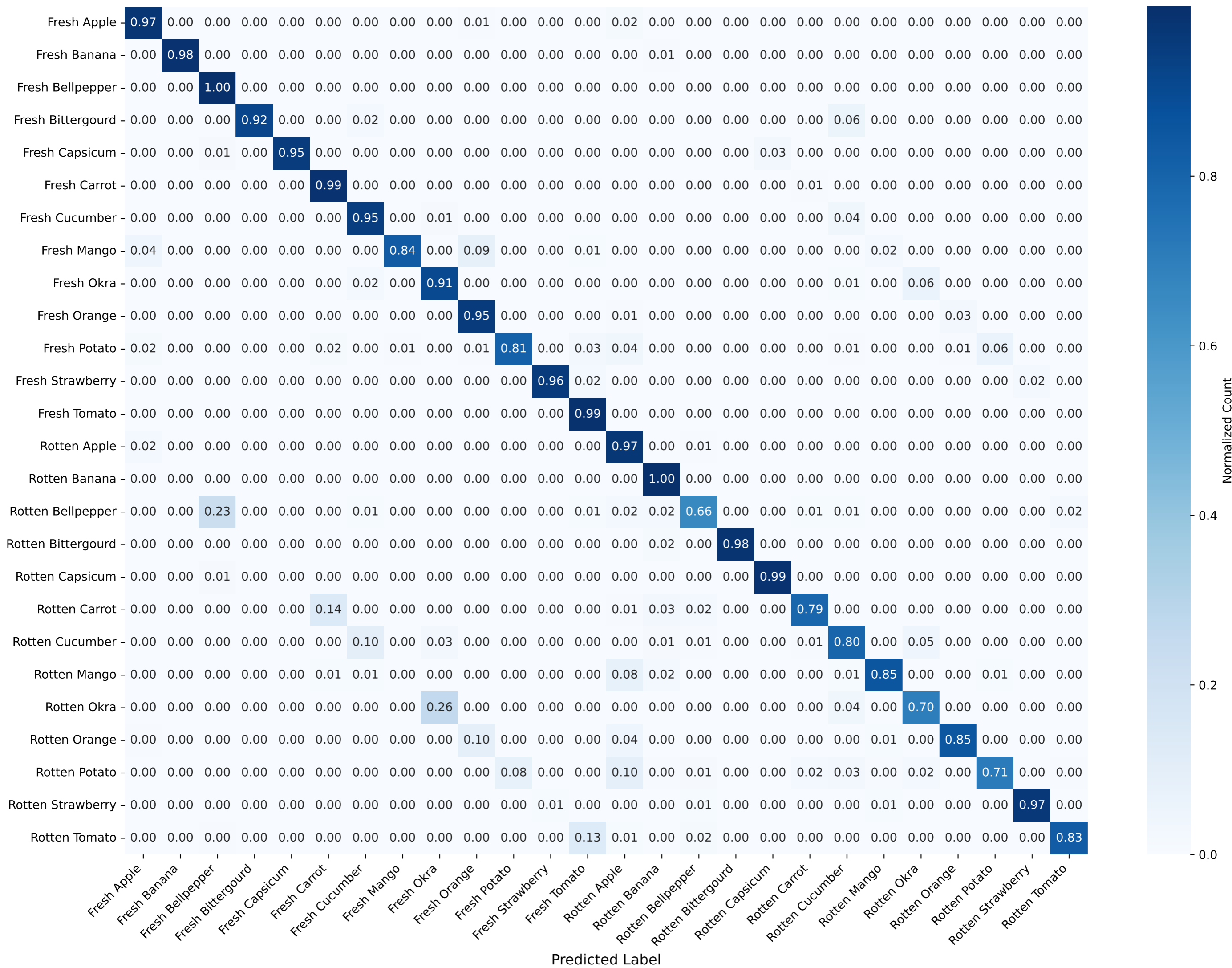
RQ5 Fig 1: Normalized Confusion Matrix - Test Set
