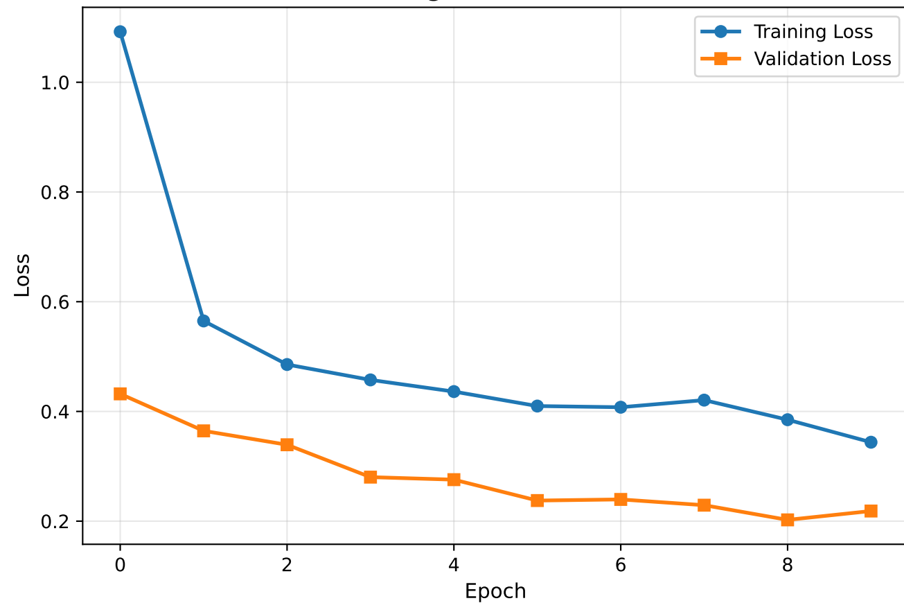
RQ2 Fig 1a: Loss Curves
