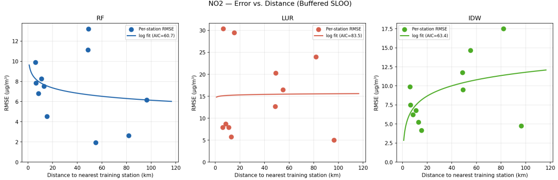
Figure 2: \text{NO}_2 error-distance decay curves under buffered SLOO, for Random Forest (left), linear regression (centre), and IDW (right). Points represent per-station RMSE. The fitted curve uses the best-fit functional form selected by AIC (Table 6).
