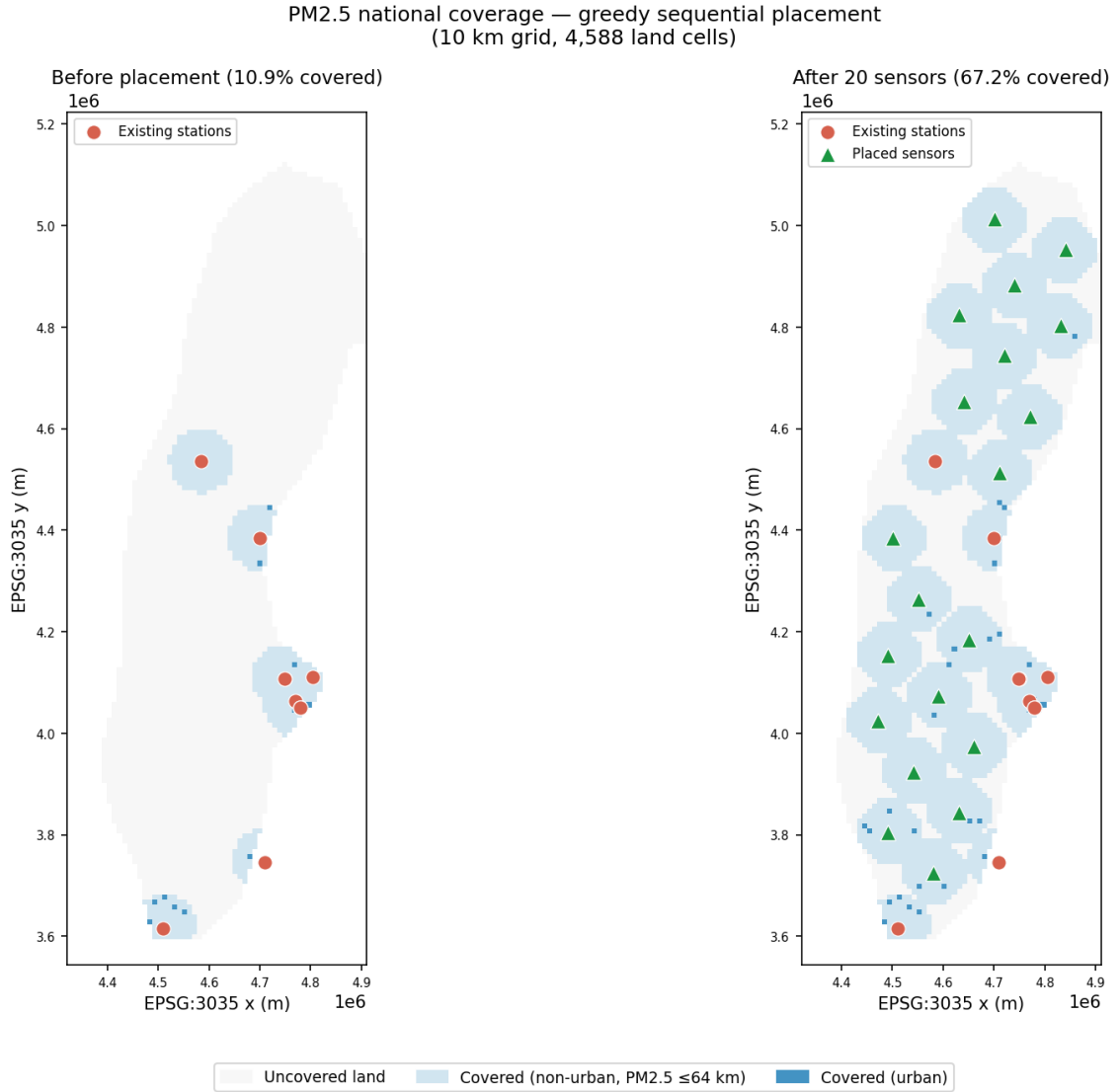
Figure 5: PM 2.5 national coverage before (left) and after (right) 20 greedy placements. Light grey cells are beyond the 64 km reliable estimation threshold; light blue cells are covered non-urban land; dark blue cells are covered urban land (CORINE 111 and 112). Red circles indicate existing stations; green triangles indicate recommended sensor locations (right panel only). Grid resolution: 10 km.
