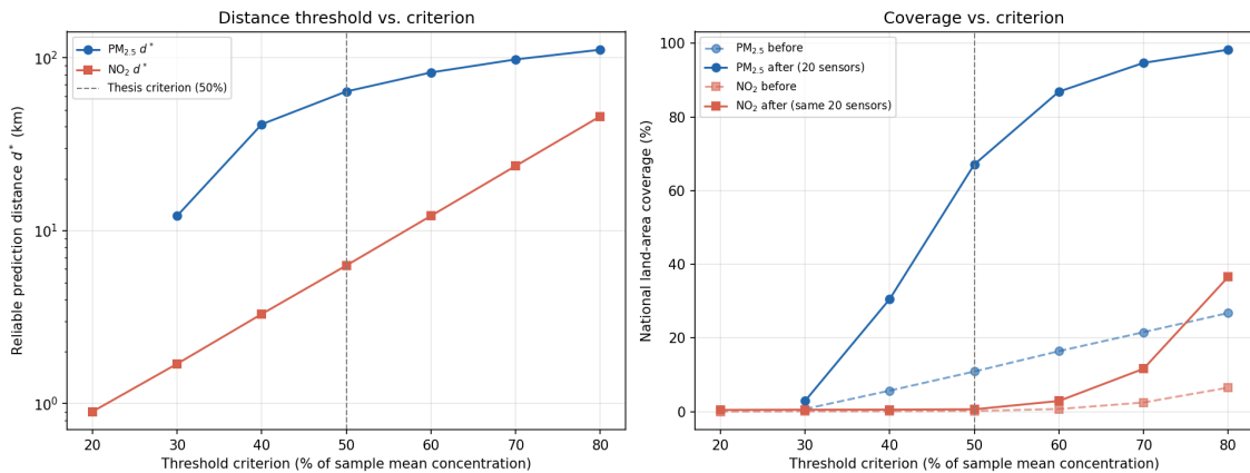
Figure 4: Sensitivity of the estimated prediction-distance threshold d^* (left) and of national PM 2.5 /NO 2 land coverage before and after the 20-sensor placement (right) to the choice of threshold criterion, swept from 20 to 80 per cent of the sample mean concentration. The dashed grey line marks the 50 per cent criterion used throughout this thesis.
