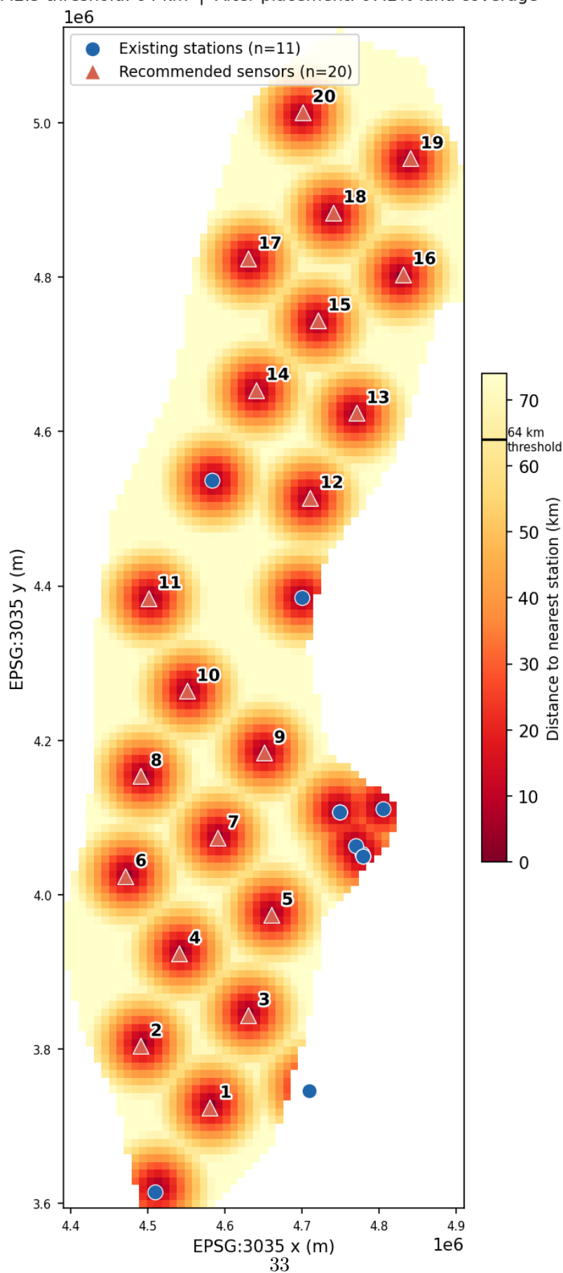
Figure 7: Distance to nearest monitoring station (km) across the Swedish national grid after greedy placement, combining the 11 existing stations and the 20 recommended sensors. The colourbar threshold at 64 km marks the PM 2.5 reliable estimation boundary. Existing
