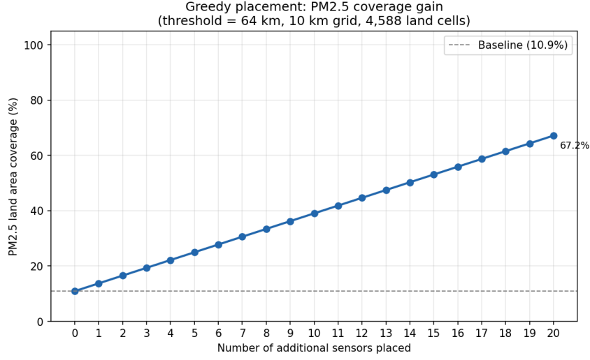
Figure 5: PM 2.5 land area coverage as a function of the number of additional sensors placed by the greedy sequential algorithm. The dashed line marks the baseline coverage of 10.9 % provided by the 11 existing concurrent-passing stations. Each step adds 129 grid cells (12,900 km 2 ) of new coverage.
