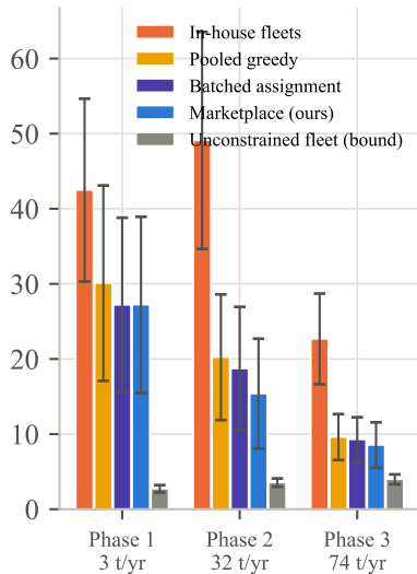
A. Urgent cargo: 90th-percentile delay (h)
