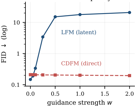
Generation quality
