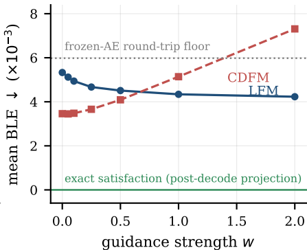
Constraint satisfaction
