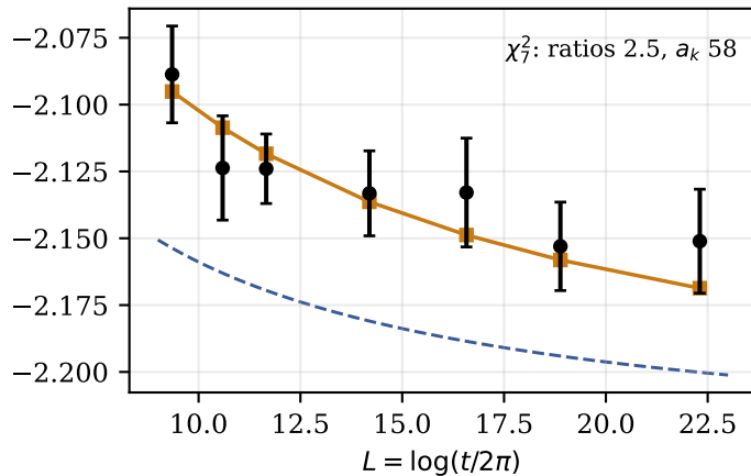
b = 0: \kappa_3(\log|\zeta|)
