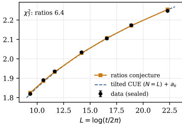
b = 0: \kappa_2(\log|\zeta|)
