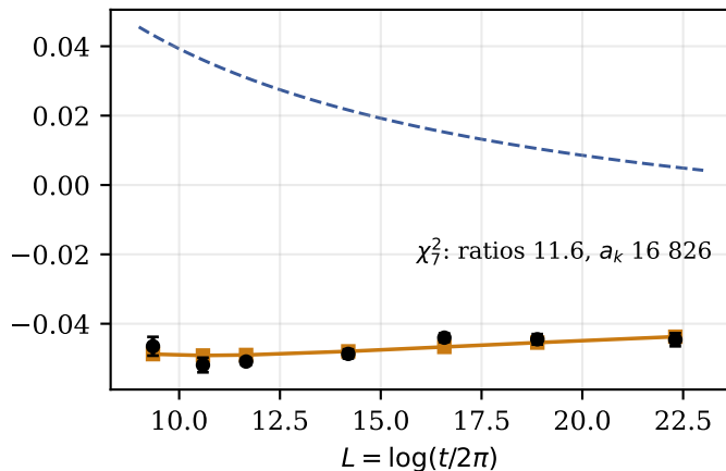
b = 1: \kappa_3(\log|\zeta'(\rho)|)
