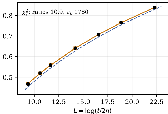
b = 1: \kappa_2(\log|\zeta'(\rho)|)
