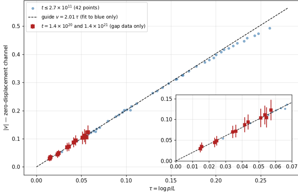
FIGURE 2. The zero-displacement transmission |v| against \tau = \log p/L (previous convention on both axes of the comparison; complete-basis re-measurement pending). Blue: measurements at t \leq 2.7 \times 10^{11} . Red: the twelve gap-only measurements at t = 1.4 \times 10^{20} and 1.4 \times 10^{21} . Dashed: the linear guide fitted only to the blue points. Inset: the small- \tau region.
