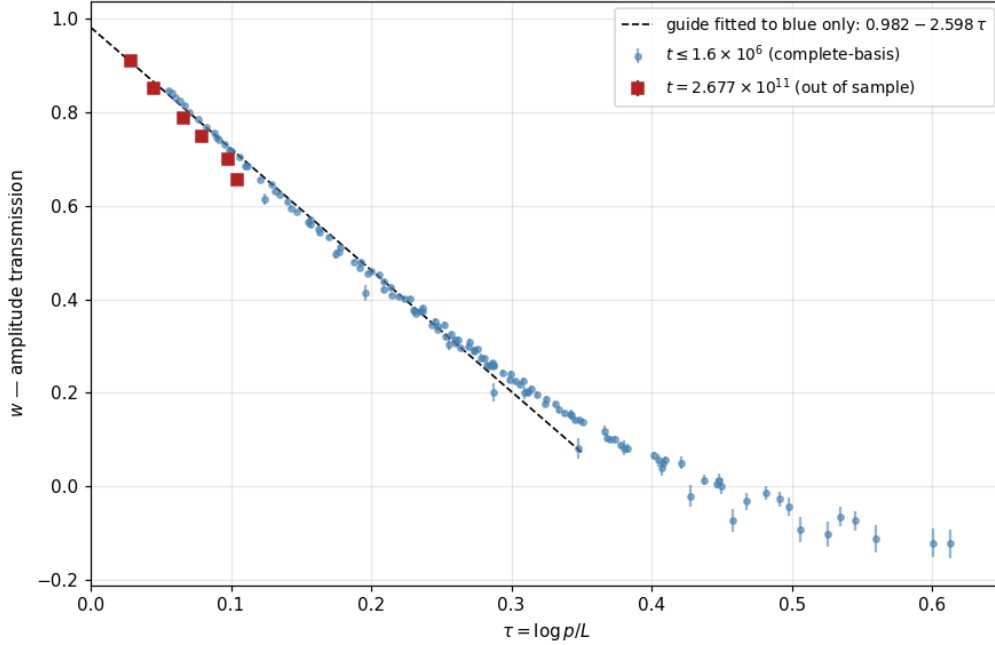
FIGURE 1. The amplitude-channel transmission w against \tau = \log p/L , complete-basis convention. Blue: the 132 measurements at t \leq 1.6 \times 10^6 . Red: the six out-of-sample measurements at t = 2.677 \times 10^{11} . Dashed: the linear guide fitted only to the blue points.
