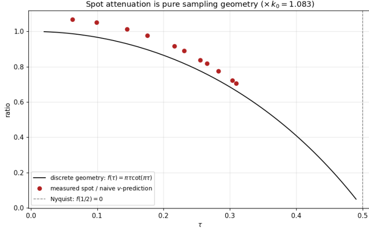
FIGURE 2. Spot attenuation against the naive v -based prediction collapses onto the discrete sampling geometry \pi\tau \cot(\pi\tau) , times the flat constant k_0 = 1.083 \pm 0.007 .
