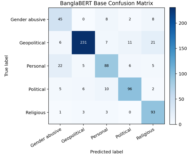
Fig. 6. Confusion matrix for BanglaBERT Base on the test set.
