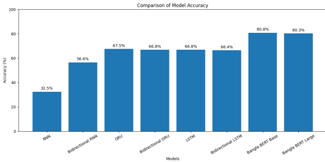
Fig. 5. Accuracy comparison of deep learning models on the Bengali hate and offensive speech dataset.
