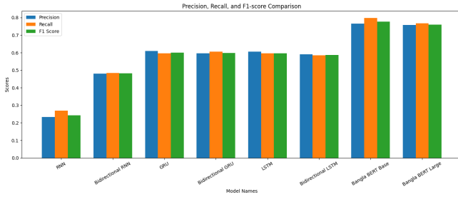
Fig. 4. Comparison of macro-averaged precision, recall, and F1-score across different models.
