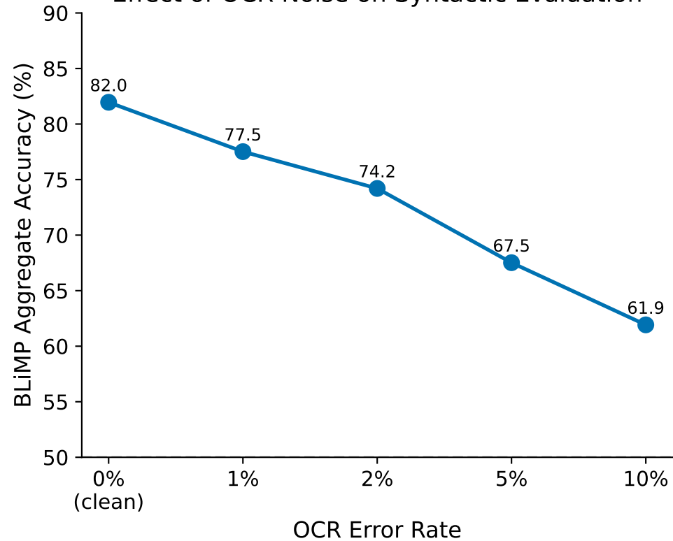
Effect of OCR Noise on Syntactic Evaluation
