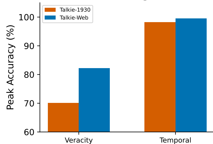
Probing
