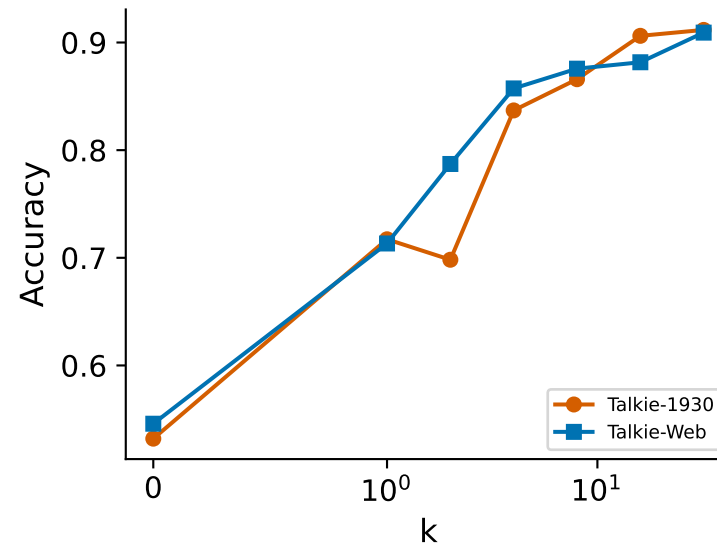
ICL (SST-2)
