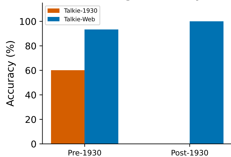
Knowledge Boundary
