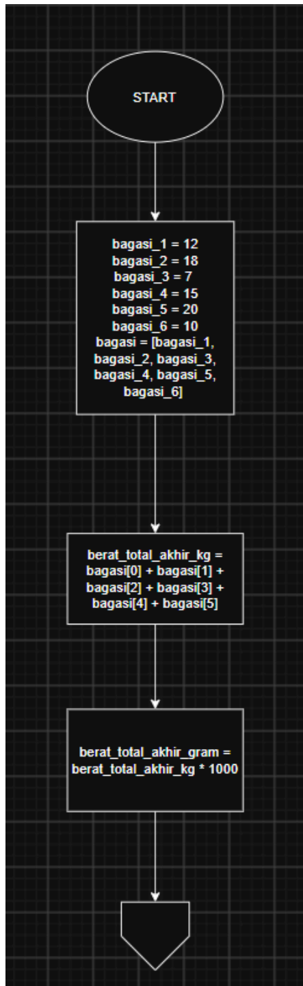
Gambar 1.1 Flowchart
