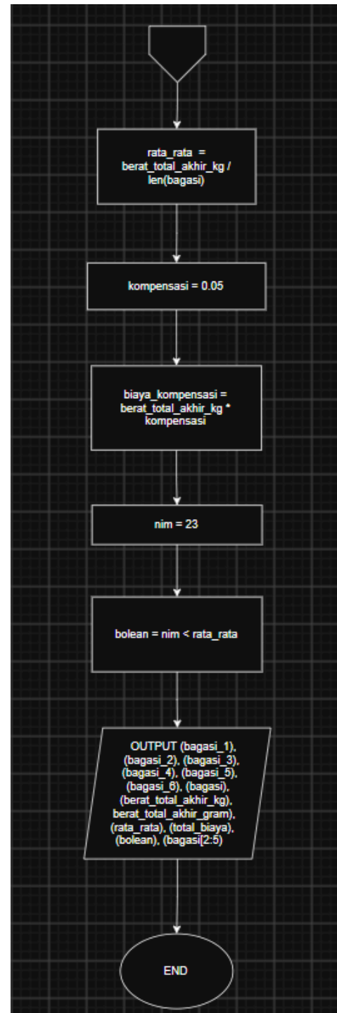
Gambar 1.2 Flowchart
