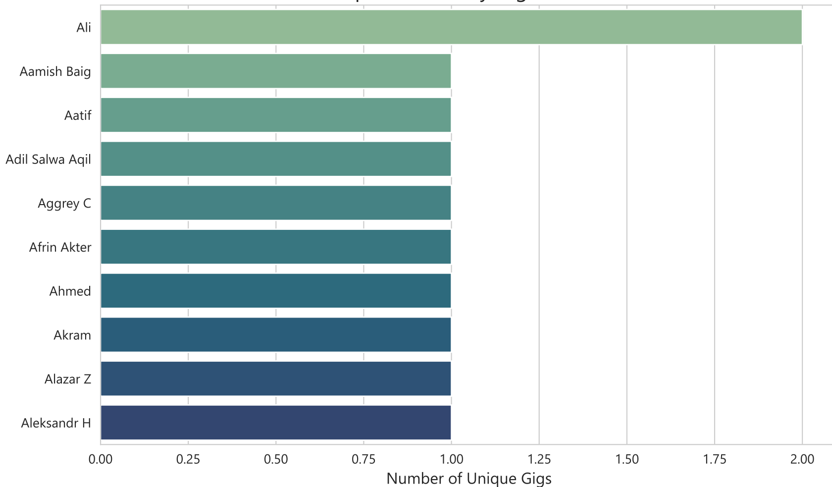
Top 10 Sellers by Gig Volume
