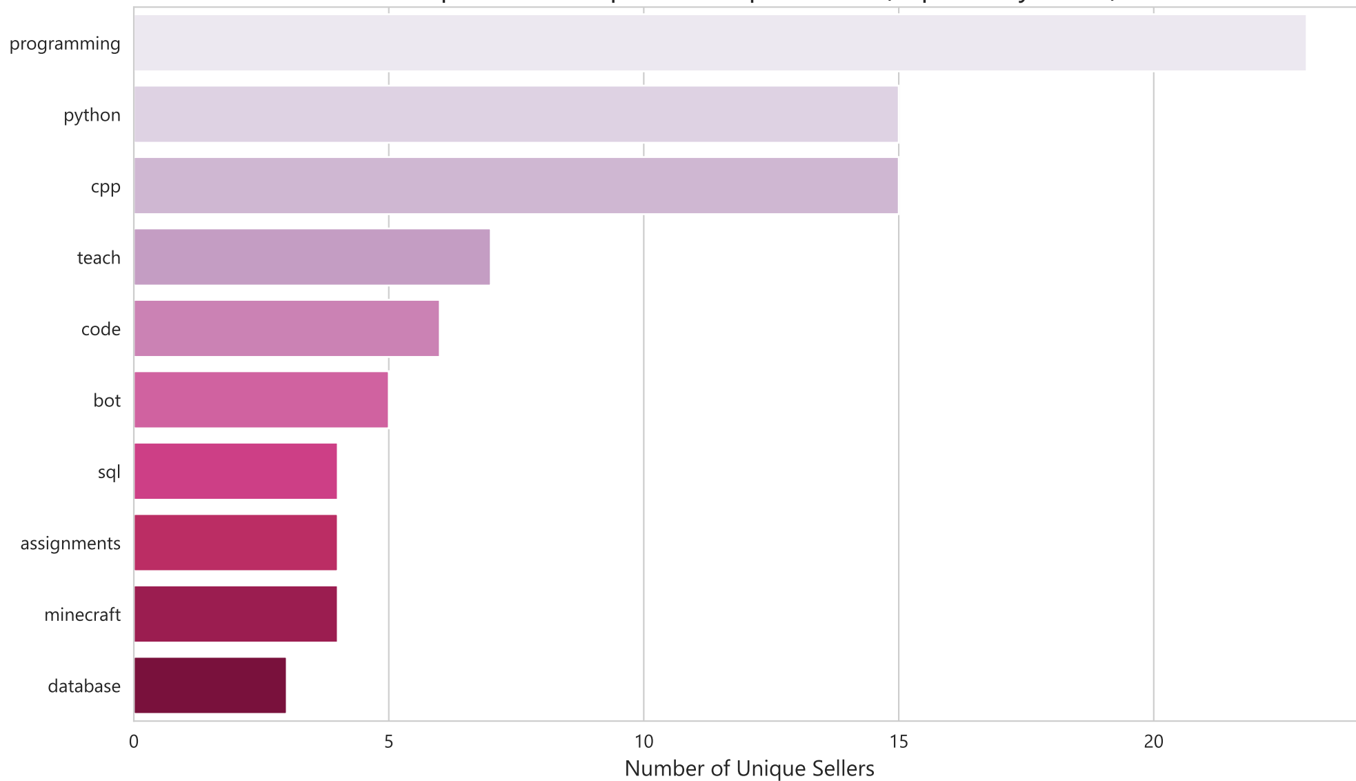
Competition: Unique Sellers per Niche (Top 10 Keywords)
