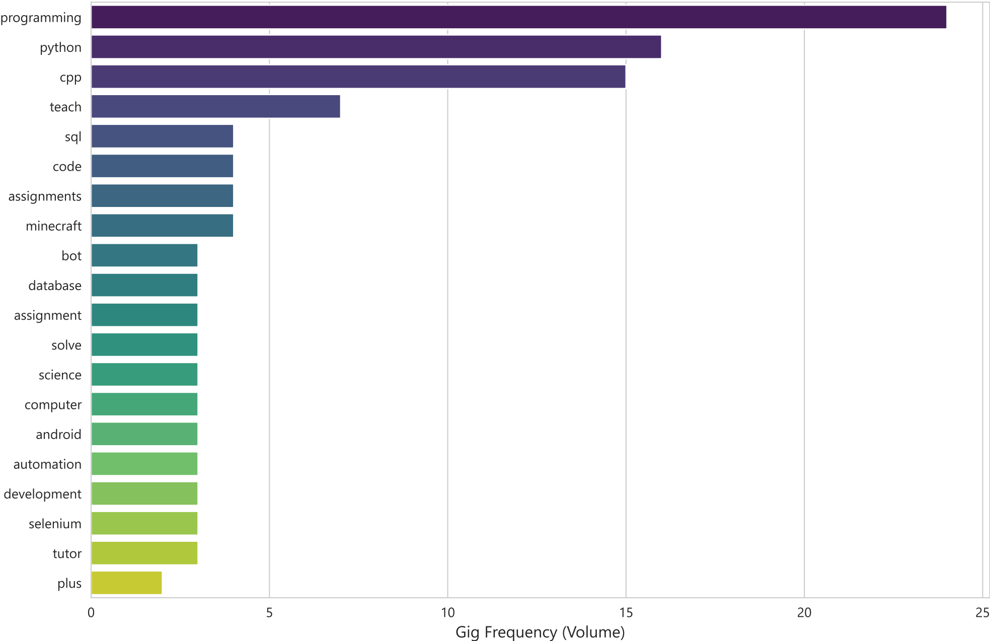
Top 20 Technical Keywords by Gig Volume for 'Java'
