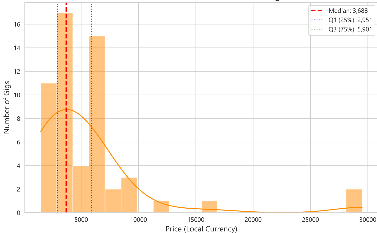
Market Price Distribution (95% of Gigs)
