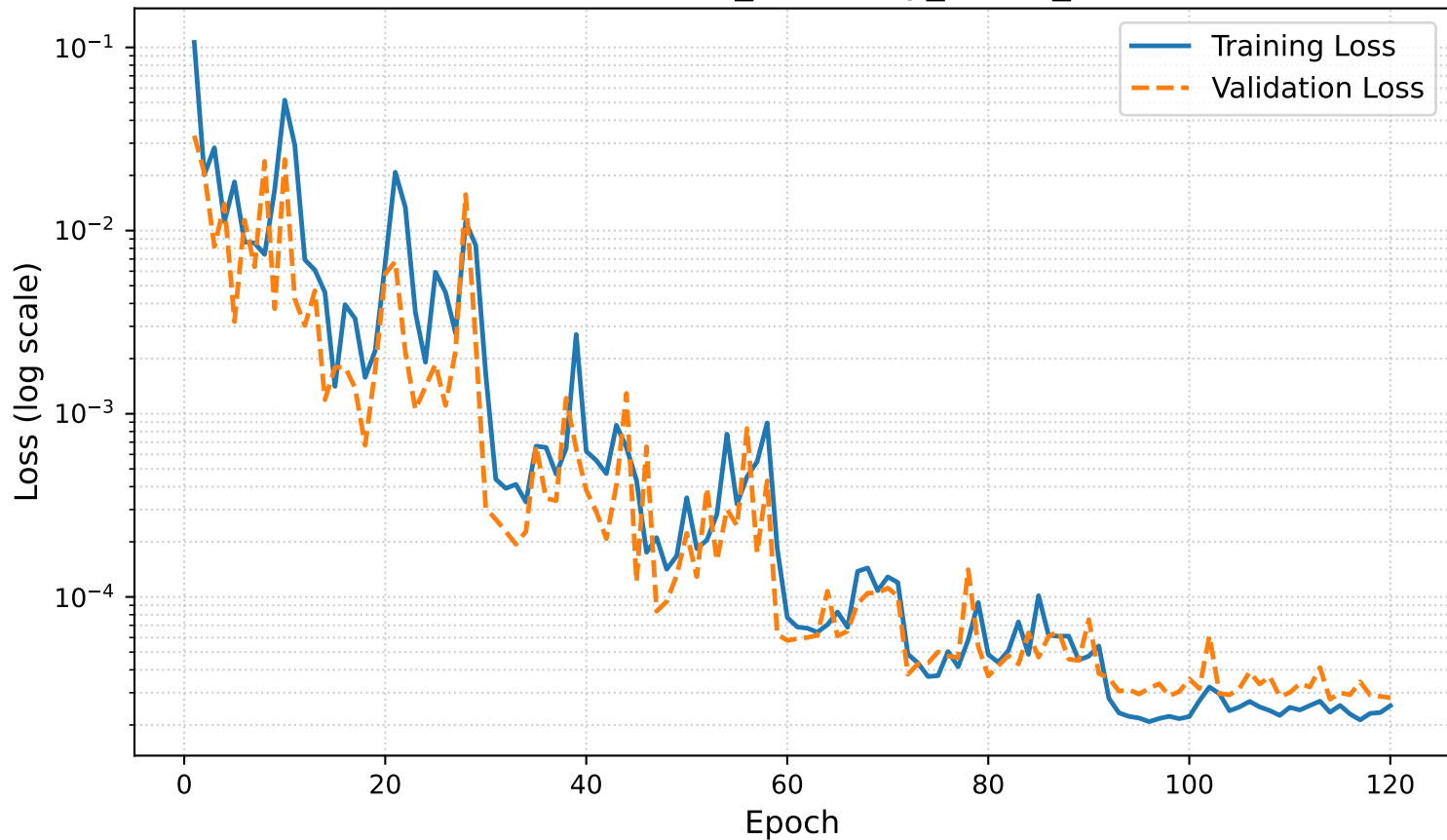
Loss Evolution: flux_boundary_train8_bottom
