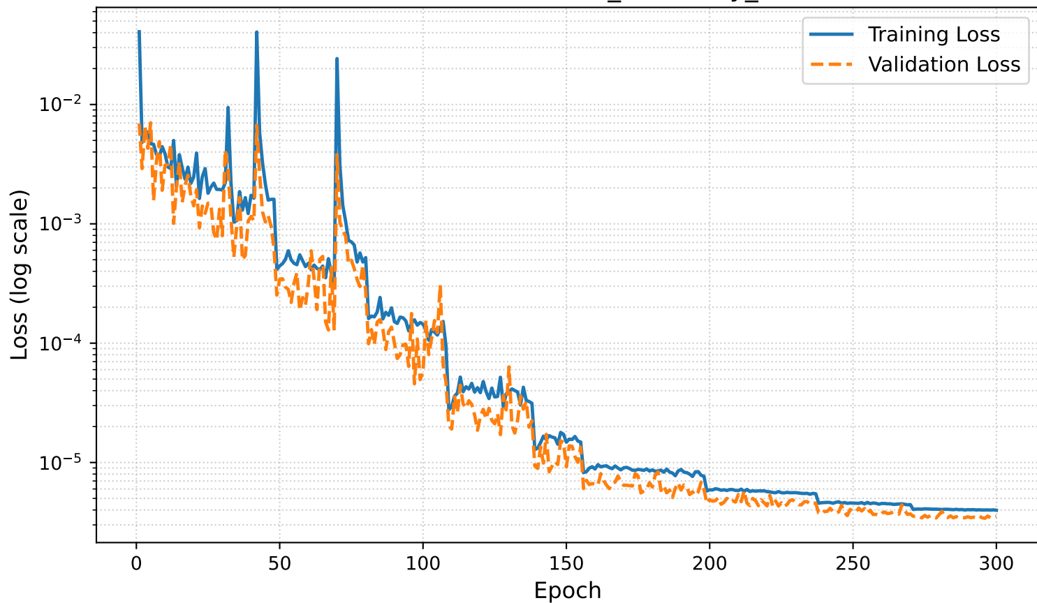
Loss Evolution: solution_boundary_train8
