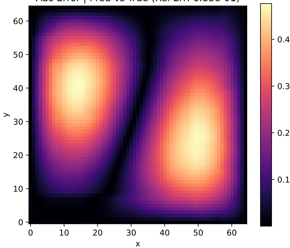
Abs Error | Pred vs True (Rel Err: 6.83e-01)
