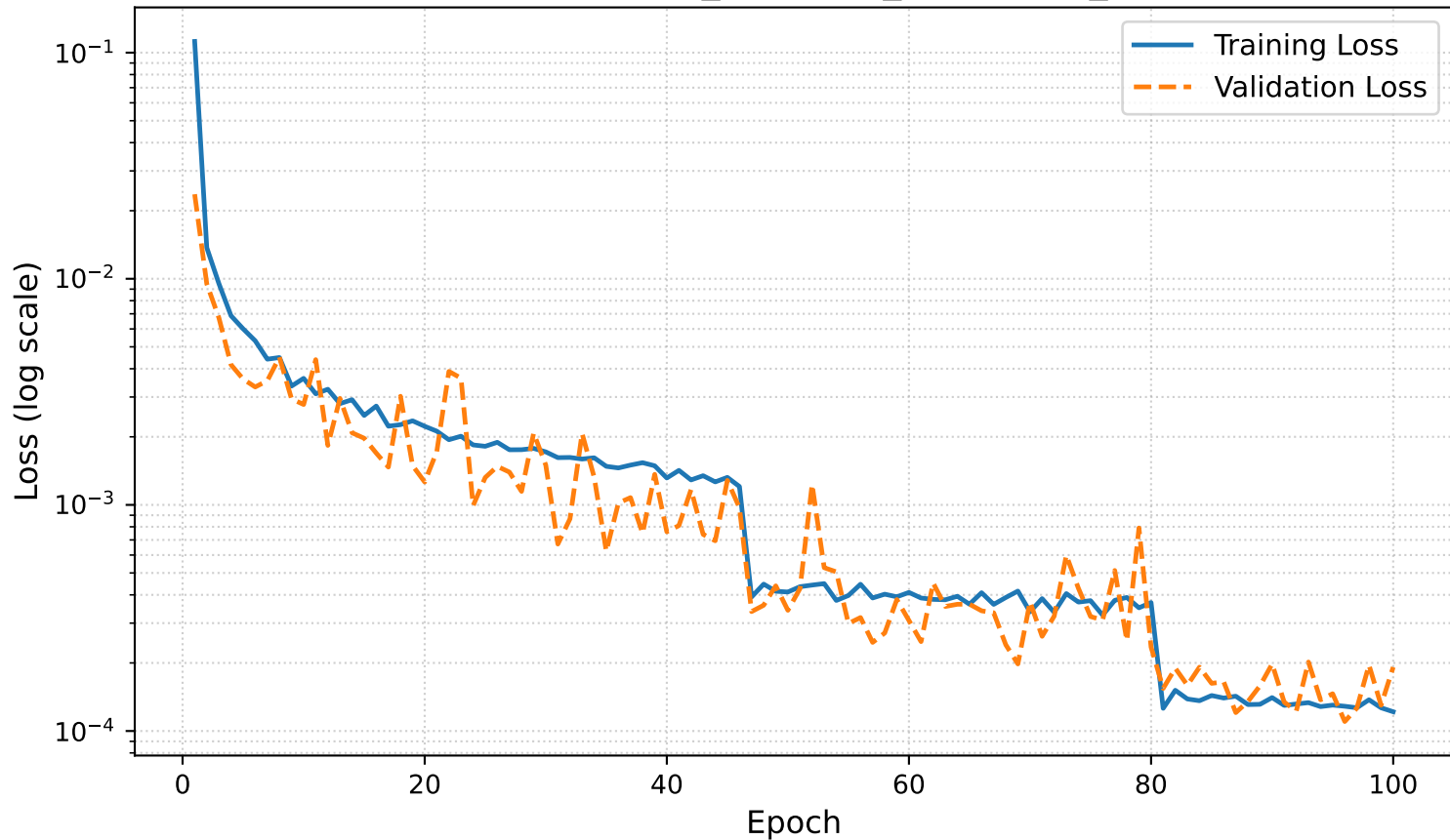
Loss Evolution: flux_internal6_hyperpara_bottom
