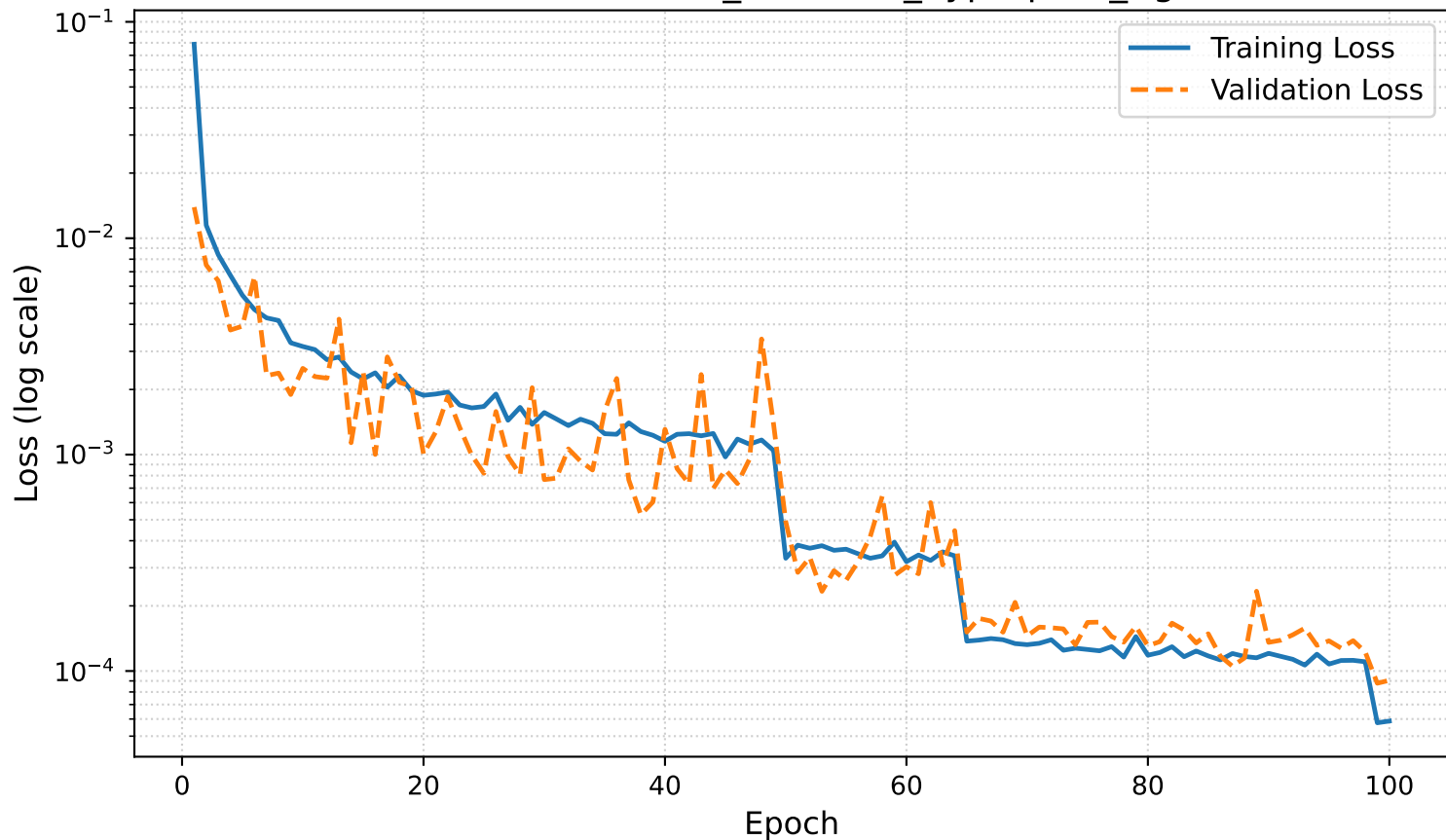
Loss Evolution: flux_internal6_hyperpara_right
