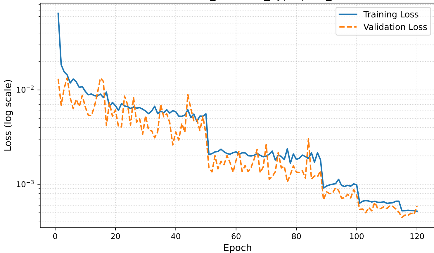
Loss Evolution: flux_internal8_hyperpara_bottom
