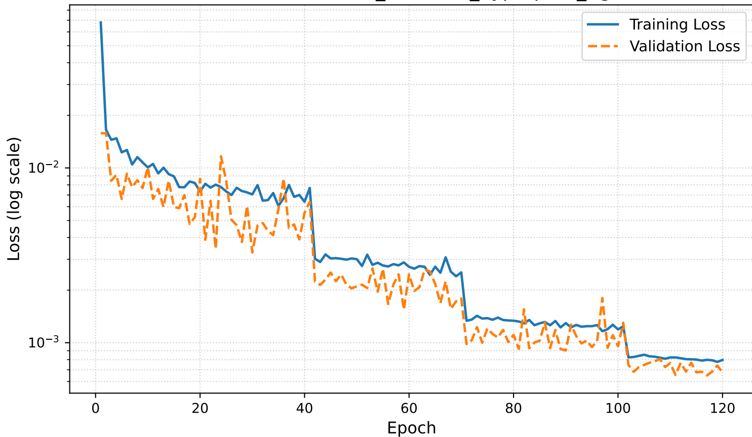
Loss Evolution: flux_internal8_hyperpara_right
