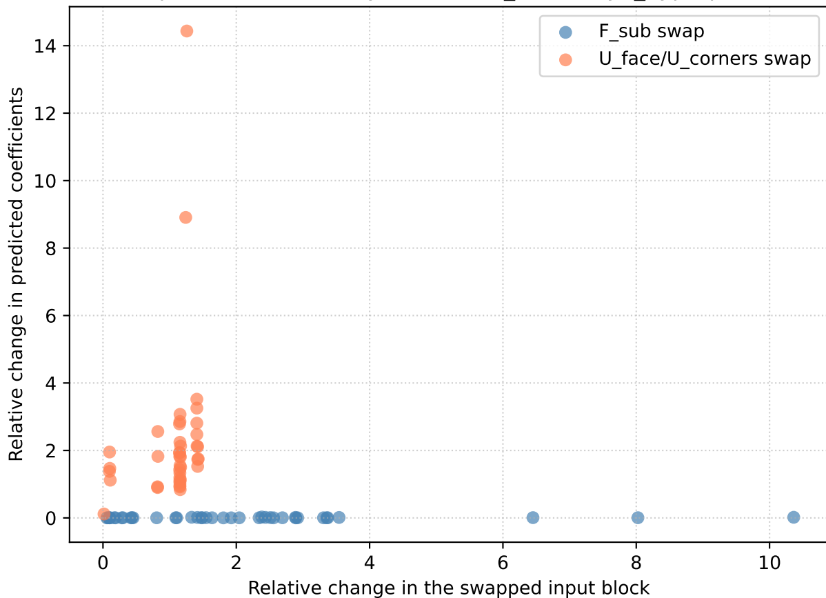
Input block sensitivity — solution_boundary8_hyperpara
