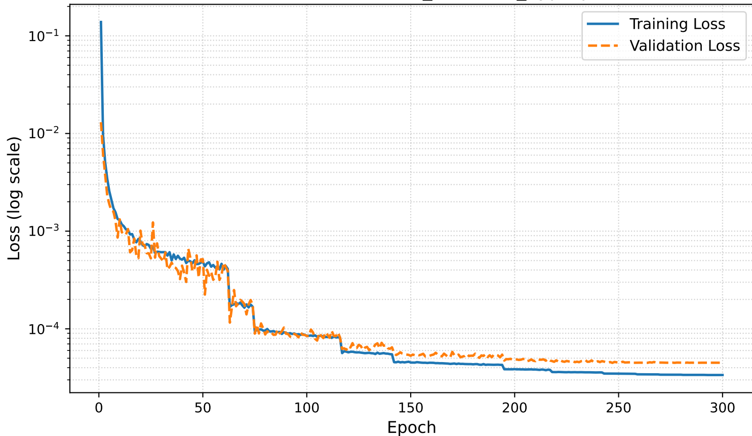
Loss Evolution: solution_internal8_hyperpara
