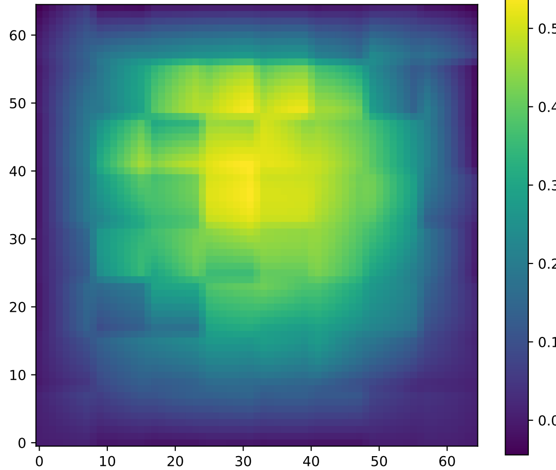
Reconstructed Prediction
