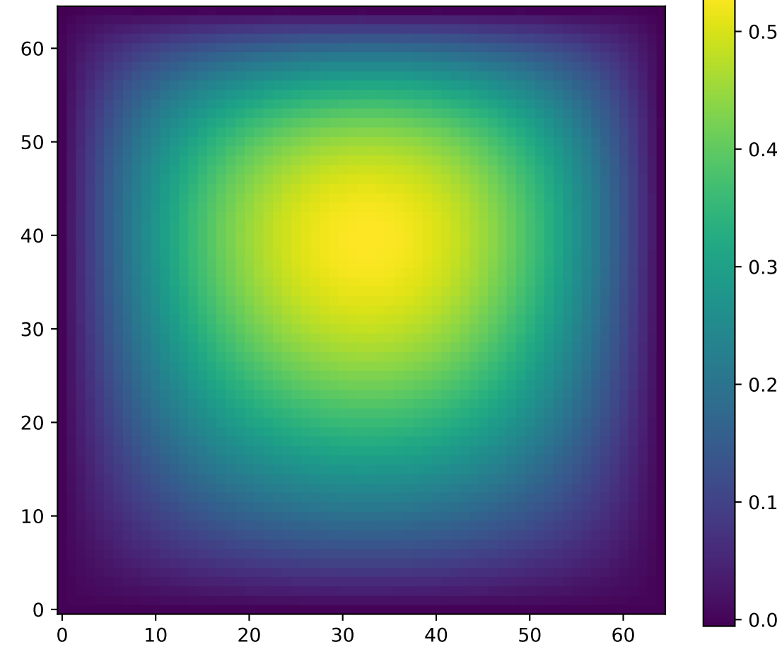
Ground Truth Physical Solution
