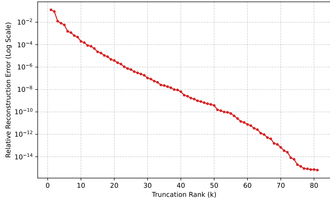
F_sub (Boundary) Error (Log Scale)
