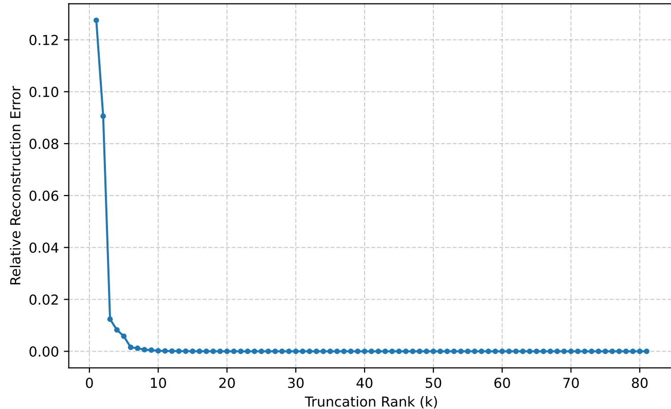
F_sub (Boundary) Error (Linear Scale)
