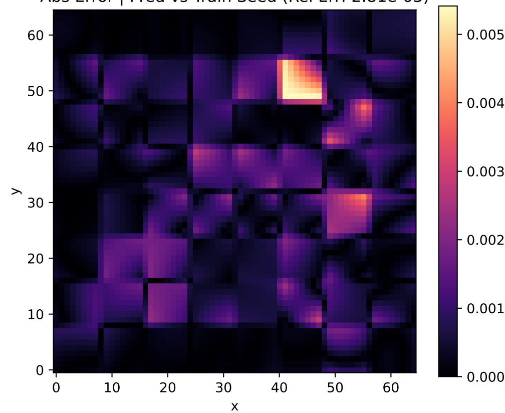
Abs Error | Pred vs Train Seed (Rel Err: 2.81e-03)
