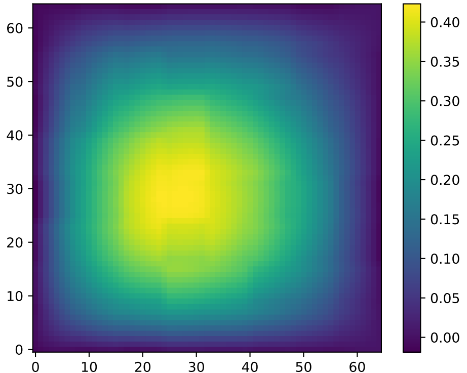
U-Net Prediction
